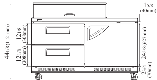
TST-60SD-18M-D2R-FB-N FRONT VIEW
