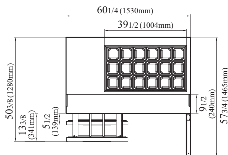
TST-60SD-18M-D2R-FB-N-LW TOP VIEW
