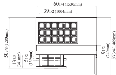
TST-60SD-18M-D2R-FB-N TOP VIEW
