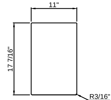
CUT-OUT SIZE
