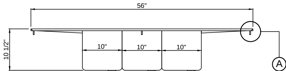
FRONT ELEVATION
