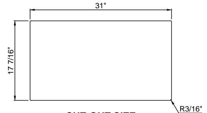
CUT-OUT SIZE
