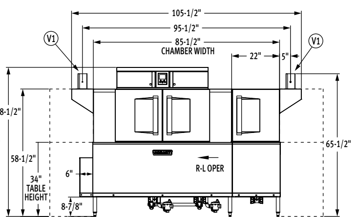
Front View Right to Left Machine
