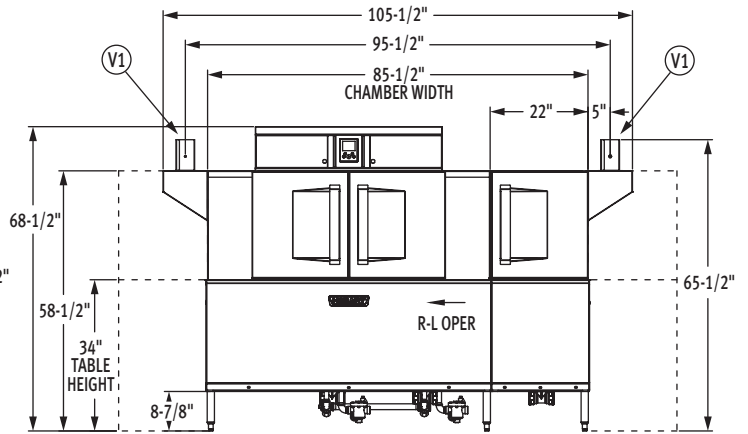
Front View Right to Left Machine
