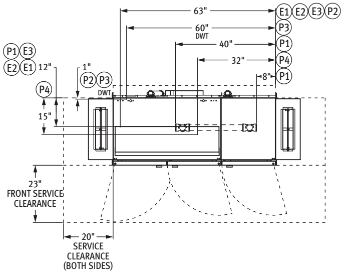
Top View Right to Left Machine
