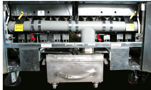
Pull out on the handle to remove the filter pan.
