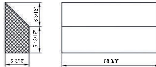
Evaporator Compartment Evaporator Compartment Capacity: 2.41 Cu Ft
