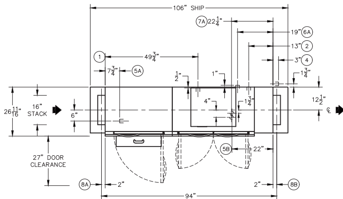
Plan View: Left to Right Model
