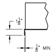
Flange Details
