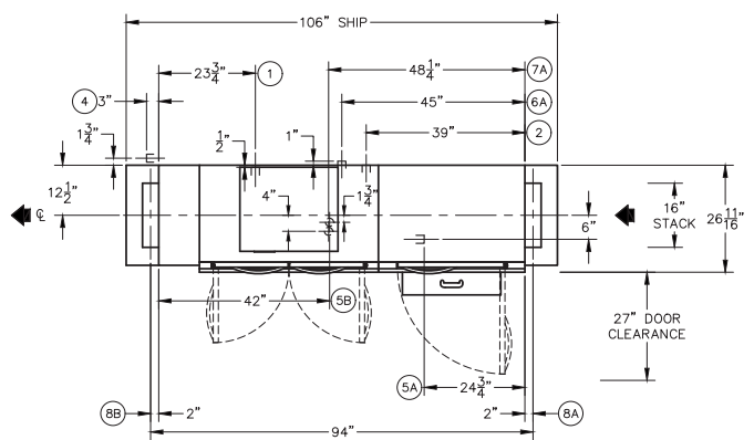
Plan View: Right to Left Model
