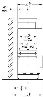
End View
