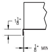
Flange Details
